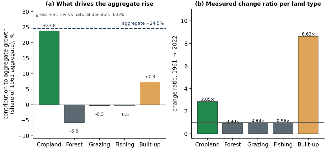
Figure 2: Measured land-type composition of the aggregate biocapacity change, National Footprint & Biocapacity Accounts (world, 1961–2022). The aggregate grew +24.5% ( \Delta \ln B = +0.219 ), yet (a) the growth is almost entirely cropland and built-up land: cropland contributes +23.8 points and built-up +7.3 points to the aggregate increase (gross +31.1 points) while forest products, grazing and fishing together contribute −6.6 points, so the components sum exactly to the aggregate growth. (b) The measured change ratios confirm the composition: cropland 2.85×, built-up 8.63×, forest products 0.90×, grazing 0.98×, fishing 0.96×. A single aggregate number therefore cannot reveal this composition; component reporting is required at every level at which an aggregate is used to summarise ecological change.
